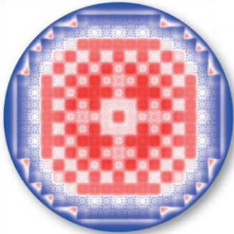
Neutronics calculation of EPR core with APOLLO 3
