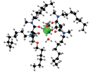
Actinide complex solvated by extraction molecul
