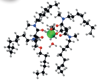
Actinide complex solvated by extraction molecule
